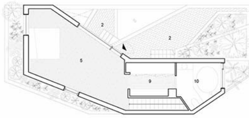
2nd floor plan 2. Terrace 5. Bedroom 9. Closet 10. SPA
